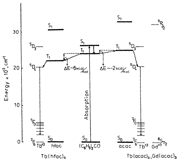
Fig. 11. Energy level diagram for the lowest excited states of benzophenone, \text{Tb}(\text{acac})_3 , \text{Gd}(\text{acac})_3 and \text{Tb}(\text{hfac})_3 [72].
