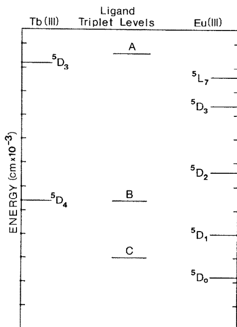
Fig. 5. Schematic energy level diagram showing relative positions of excited europium(III), terbium(III), and \beta -diketonate triplet levels.
