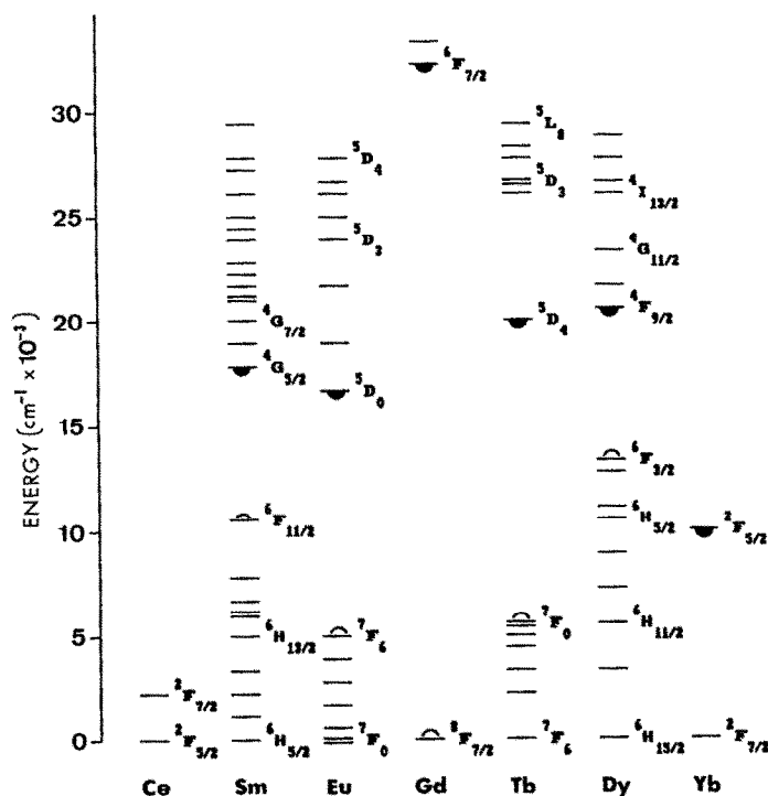
Fig. 1. Comparison of electronic energy levels for triply charged lanthanide ions ( \text{Ln}^{3+} ). Filled semicircles indicate the lowest luminescent level whereas unfilled semicircles indicate the highest level of the ground state manifold.
