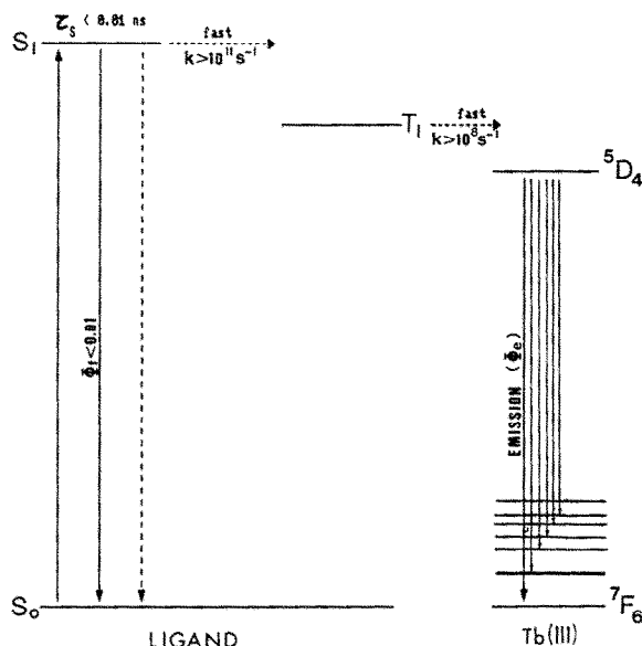
Fig. 8. Energy level diagram and known kinetic parameters for lowest excited states of terbium(III) methylsalicylate at room temperature [26]. (Although the \Phi_e and \tau values for emitting ^5D_4 level of terbium(III) methylsalicylate are not reported, appropriate values are known for chelates of the same type, e.g. \text{Tb}(\text{acac})_3 : \tau = 0.19 and 0.33 upon excitation to S_1 state of ligand and ^5D_4 level respectively, in ethanol solution at room temperature [46].)
